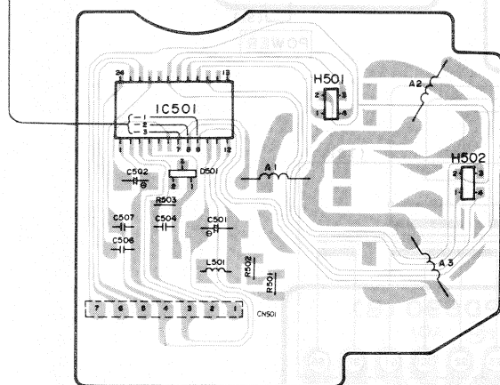
C SPINDLE MOTOR DRIVE P.C.B.
